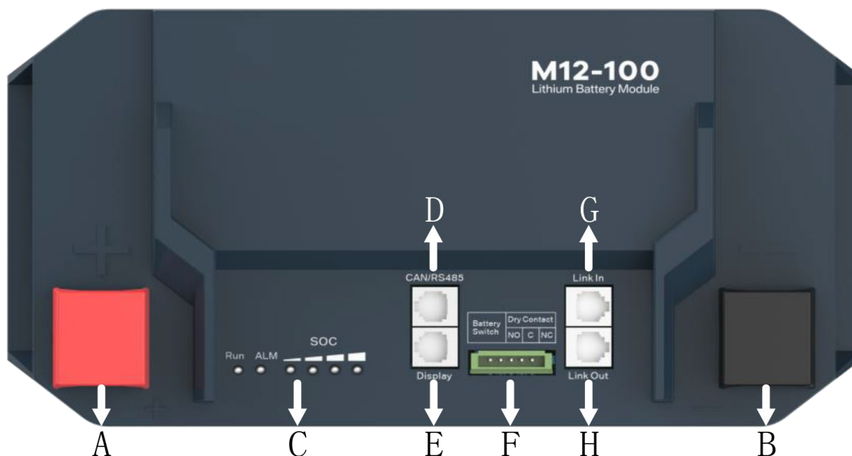
Figure 2-3 - external interfaces
