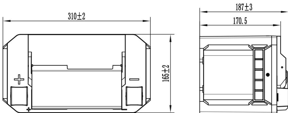
Figure 2-1 - Dimensions of M12-100
