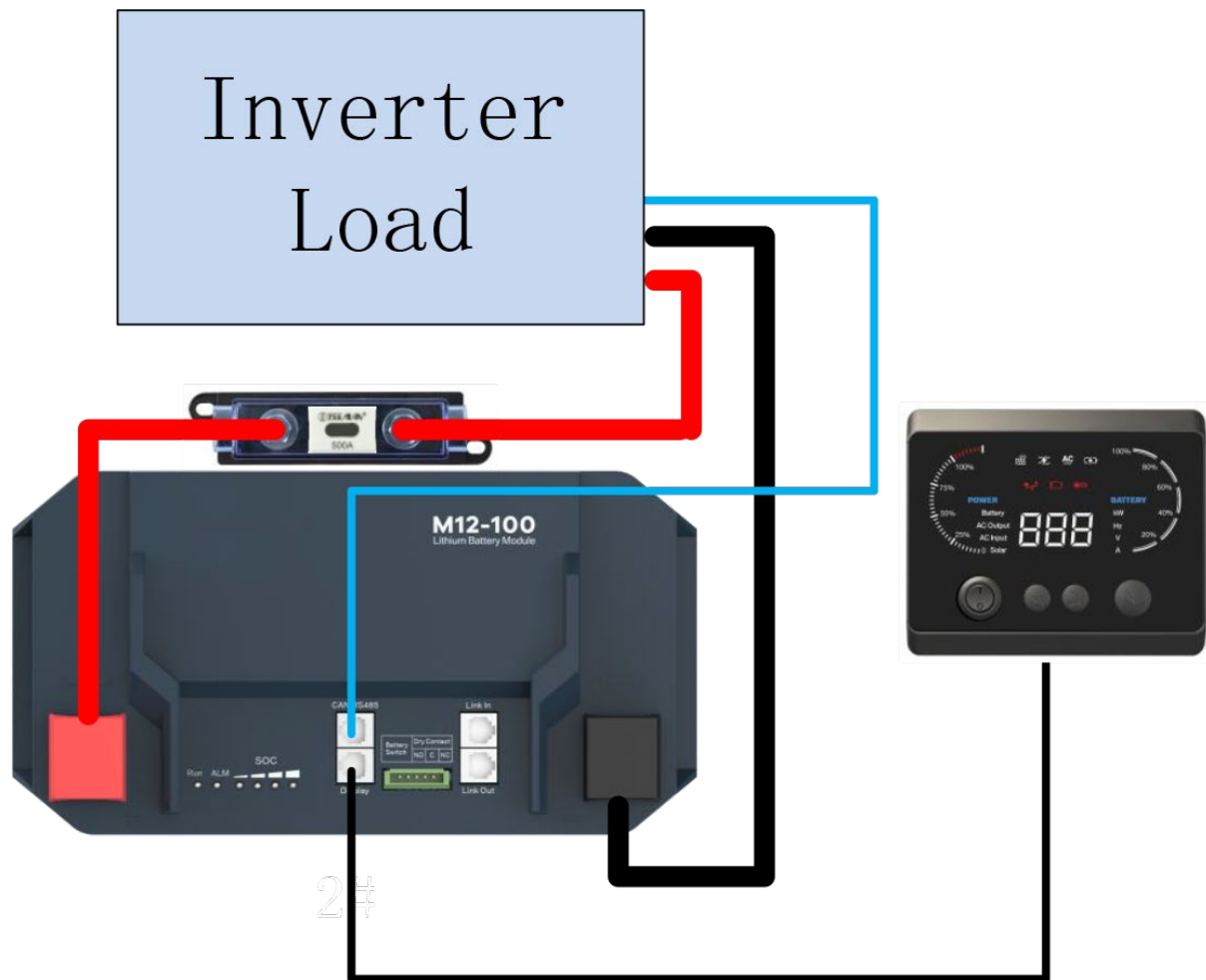
Figure 2-4 - Typical wiring diagram
